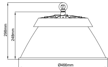
Tall Reflector
