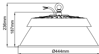
Universal Reflector
