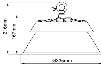
Universal Reflector
