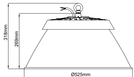
Tall Reflector
